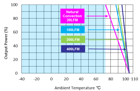
AER20-24D12, AER20-24D15, AER20-110S12, AER20-110S15, AER20-110S24, AER20-110D12, AER20-110D15 Derating Curve with Heatsink
